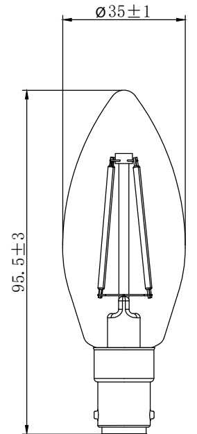
B35 with B15 base
